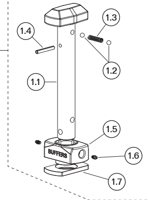
1105-3600-INNER Components
